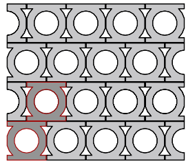
Laying Scheme 1 17.36 pieces per sqm
