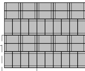
Laying Scheme 5 34.72 pieces per sqm
