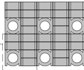
Laying Scheme 4 34.72 pieces per sqm
